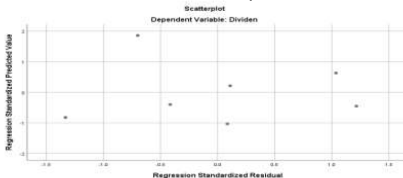
Gambar 3 Scatterplot
