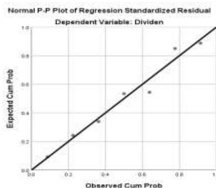
Gambar 2 P-P Plot
